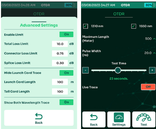
Advanced Settings
