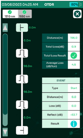
Event Map
