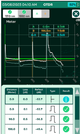
Event Table
